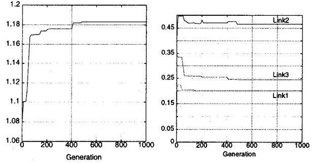
(a) Maximum Fitness (b) Results of Optimized Manipulability
