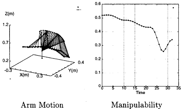
Fig. 8 Optimized 6 DOF Manipulator
