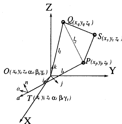
Fig. 5 Coordinate System of Modular Assembly
