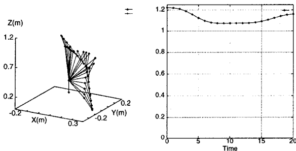
(a) Arm Motion (b) Manipulability
