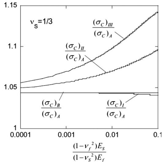
Fig. 5. Critical stress for plane strain deformation of the film/substrate system with \nu_S=1/3 . The reference is (\sigma_C)_A = (\bar{E}_f/4)(3\bar{E}_S/\bar{E}_f)^{2/3} ; (\sigma_C)_B = (\bar{E}_f/4)(3\bar{E}_S^*/\bar{E}_f)^{2/3} with \bar{E}_S^* = 4(1-\nu_S)^2\bar{E}_S/(3-4\nu_S) . Cases I–III are described in the text; (\sigma_C)_{III} is exact.
