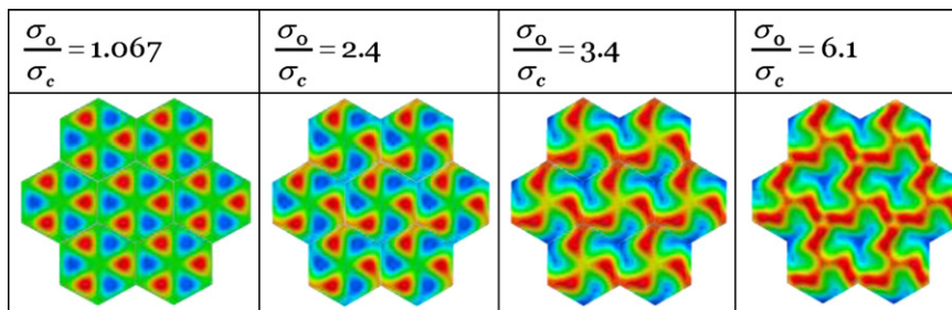
Fig. 15. Transition from a triangular mode to a asymmetric three lobed mode under increasing overstress. The result was computed with the three-dimensional finite element model using the computational cell for the triangular mode.
