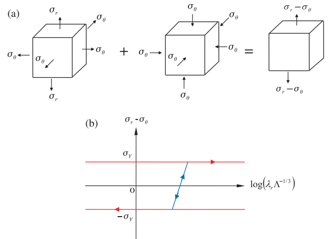
Fig. 3. (a) The state of elastic-plastic deformation of the element subject to the triaxial stresses (\sigma_r, \sigma_\theta, \sigma_\theta) is the same as that of the element subject to a uniaxial stress (\sigma_r - \sigma_\theta) . (b) The uniaxial stress-strain relation in terms of the stress (\sigma_r - \sigma_\theta) and the true elastic-plastic strain \log(\lambda_r \Lambda^{-1/3}) .
