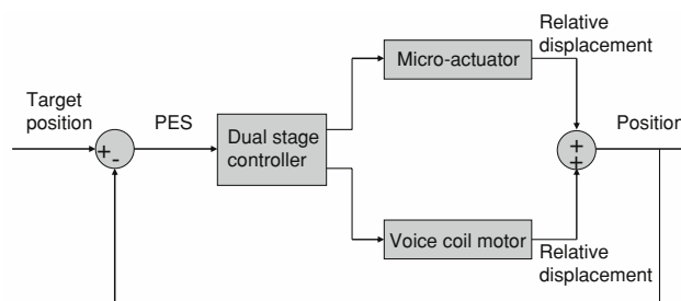
Fig. 2 Schematic of the dual stage actuator tape head concept
