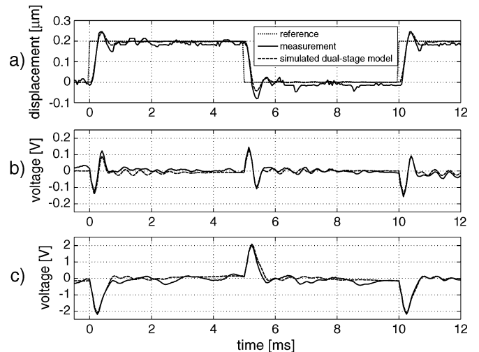
Fig. 15. Implemented controller.
