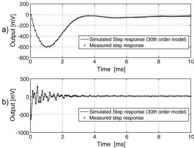
Fig. 5. Time domain validation using step response data for (a) voice coil motor model G_{VCM}(q) and (b) micro-actuator model G_{PZT}(q) .
