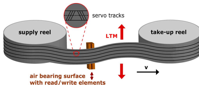
Fig. 1. Schematic of a typical tape transport.
