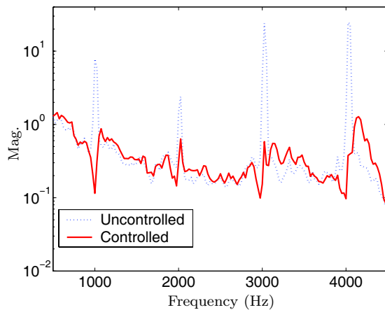
Fig. 11. Measured power spectral density of the pick-up microphone signal before (dotted) and after (solid) feedback based active noise control.
