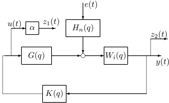
Fig. 6. The two block problem with an internal model that is used for optimal control design.
