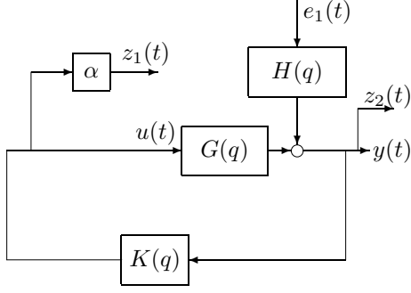
Fig. 5. Standard H_2 optimal control two-block problem, where H(q) is the noise model and \alpha is the control weighting.
