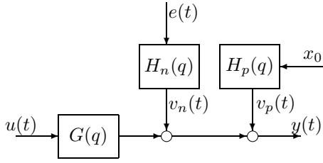
Fig. 4. Block diagram of additive periodic and non-periodic disturbance modeling.
