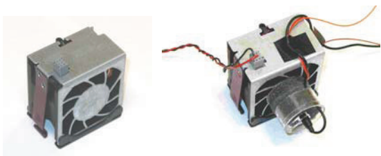
Fig. 1. Left: Server cooling fan. Right: ANC system used to cancel unwanted fan noise.
