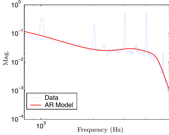
Fig. 7. Bode amplitude plot of spectral estimate of pick-up microphone signal (dotted) and AR model \|H_n(q)\|^2 \lambda (solid).
