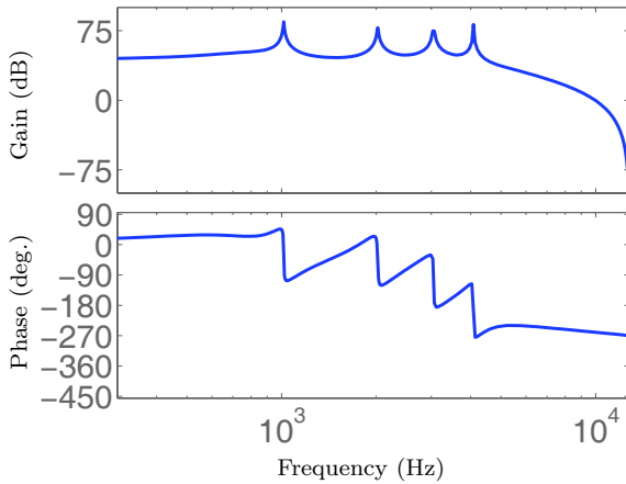
Fig. 8. The bode response of the internal model W_i(q) used to cancel periodic disturbances.
