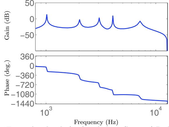
Fig. 9. Amplitude (top) and phase (bottom) Bode response of the 10th order feedback active noise control algorithm.
