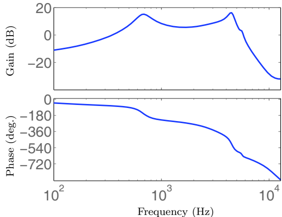
Fig. 2. Amplitude (top) and phase (bottom) Bode plot of the discrete time model G(q) used to capture the dynamics between the speaker and the pick-up microphone.
