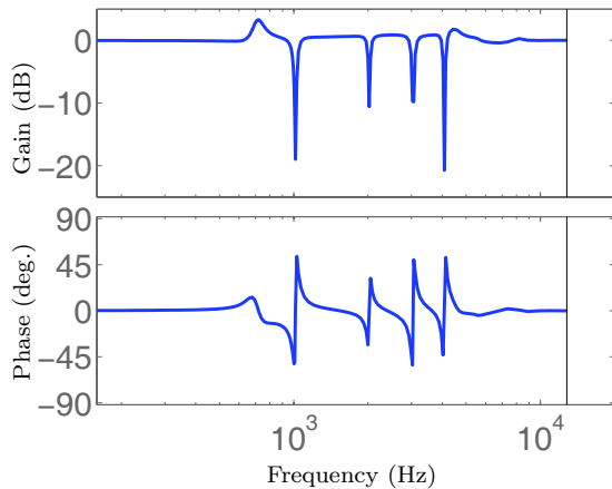
Fig. 10. Amplitude (top) and phase (bottom) Bode response of the designed sensitivity function S(q) given in (12).
