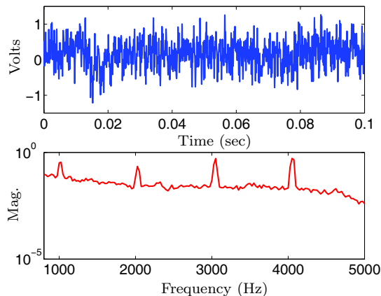
Fig. 3. Pick-up microphone data: time trace (top) and spectral estimate (bottom).
