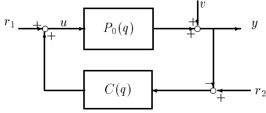
Fig. 1: Closed-loop configuration.
