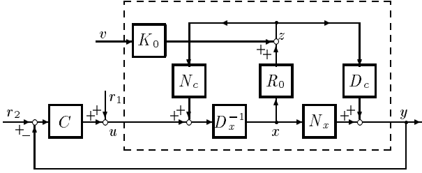
Fig. 2: Dual Youla-representation of the data generating system.
