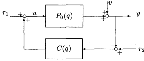
Fig. 1: Closed-loop configuration.
